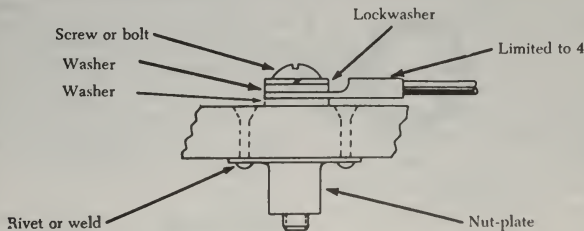
FIGURE 4-115. Nut-plate bonding or grounding to flat surface.
